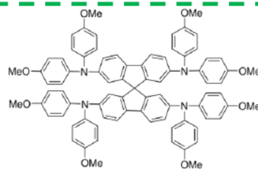
Spiro-OMeTAD
