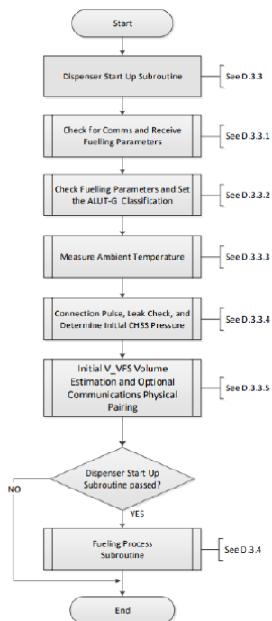
Figure D.1 High-level flow chart for the ALUT-G fuelling protocol
